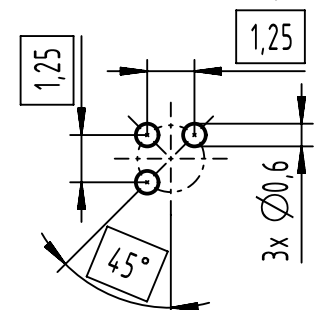
A (5:1) recommend PCB layout
